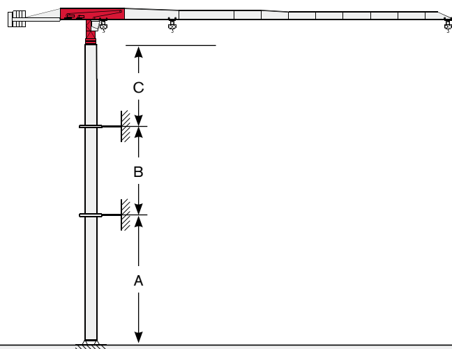
Tower: TS16 - H 200m (C25)
